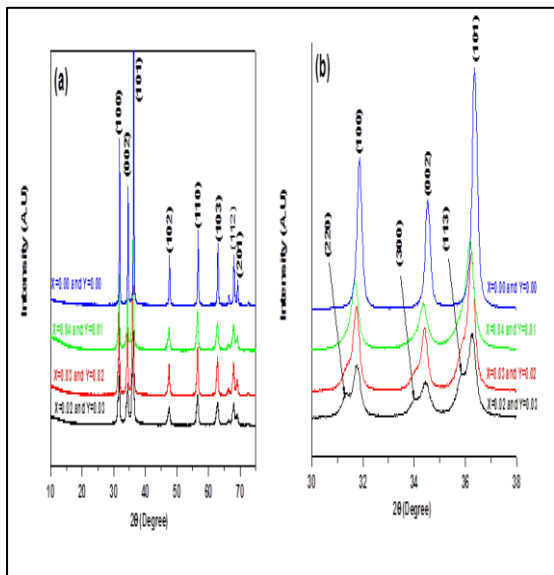
Fig 1(a): XRD patterns of Un Doped ZnO and Co(x = 0.00, 0.04, 0.03, 0.02) and Al(y = 0.00, 0.01, 0.02, 0.03) Doped ZnO Nanostructured Films and (b) XRD Patterns of Un Doped ZnO and Co(x = 0.00, 0.04, 0.03, 0.02) and Al(y = 0.00, 0.01, 0.02, 0.03) Doped ZnO Nanostructured Films, Only in the Detection Angle Range of the Preferred Orientations for Better Comparability.
