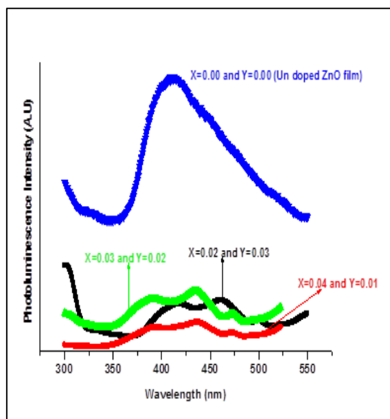
Fig 3: Photoluminescence Emission Spectra of Undoped ZnO Film and Co(x = 0.04, 0.03, 0.02) and Al(y = 0.01, 0.02, 0.03) Doped ZnO Nanostructured Films for Better Comparison of Intensity of Photoluminescence.
