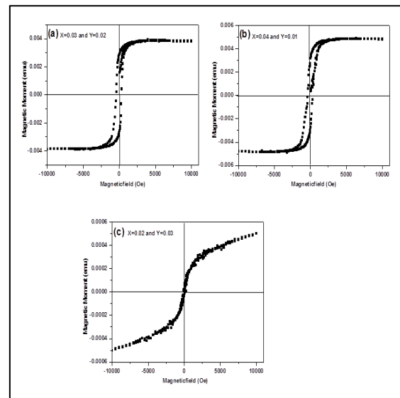
Fig 4(a-c): Room Temperature Field vs Magnetization (M-H) Loop Showing Hysteresis of the Co(x = 0.04, 0.03, 0.02) and Al(y = 0.01, 0.02, 0.03) Doped ZnO Nanostructured Films, (a) Co(x = 0.03) and Al(y = 0.02) Doped ZnO Film, (b) Co(x = 0.04) and Al(y = 0.01) Doped ZnO Film, (c) Co(x = 0.02) and Al(y = 0.03) Doped ZnO.
