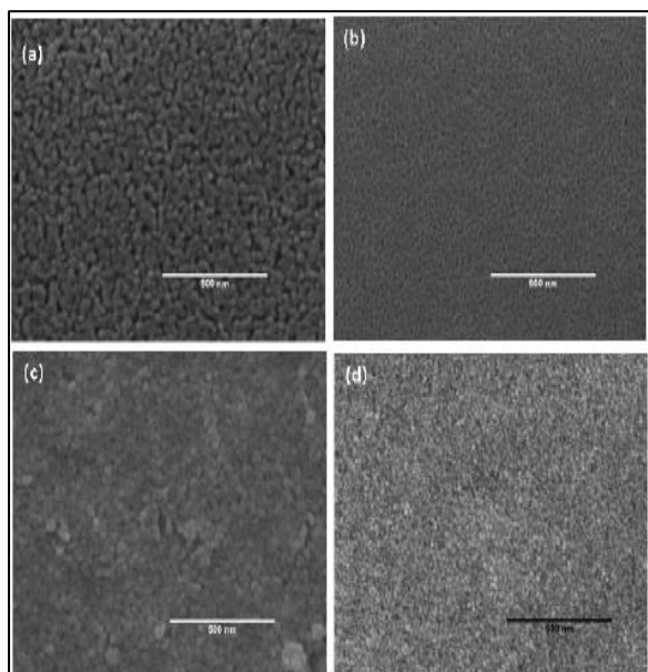
Fig 2(a-d): SEM Surface Morphology of Undoped ZnO and Co(x =0.00, 0.04, 0.03, 0.02) and Al(y = 0.00,0.01, 0.02, 0.03) Doped ZnO Nanostructured Films, (a) Undoped ZnO Film, (b) Co(x = 0.02) and Al(y = 0.03) Doped ZnO Film, (c) Co(x = 0.03) and Al(y = 0.02) Doped ZnO Film, (d) Co(x = 0.04) and Al(y = 0.01) Doped ZnO Film
